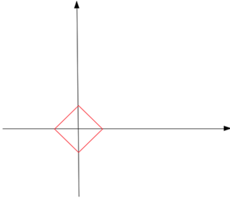
Figure 5: l^1 -norm shape
