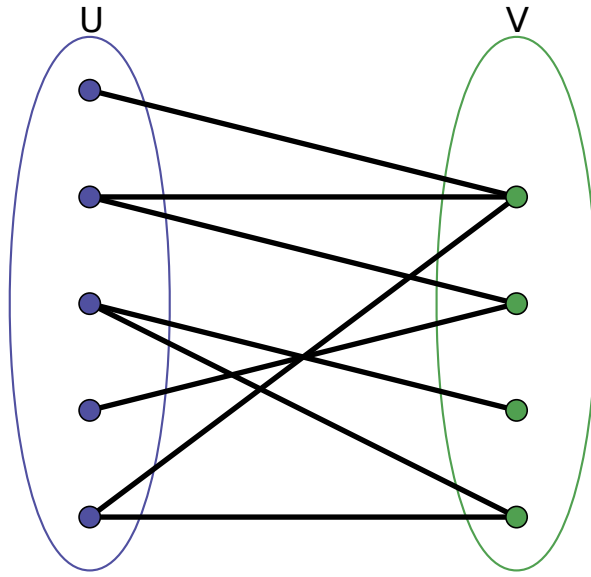
Figure 2.1: A simple bipartite graph
